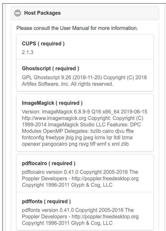
Figure 4.162. Admin Web App: About - Host Packages - 1/3
