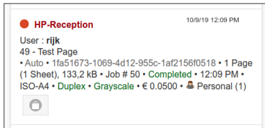
Figure 4.142. Admin Web App: Document - IPP Routing
