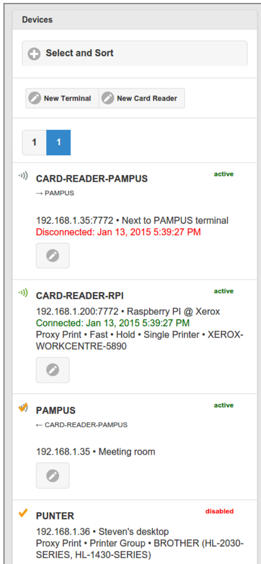
Figure 4.72. Admin Web App: Device - List
