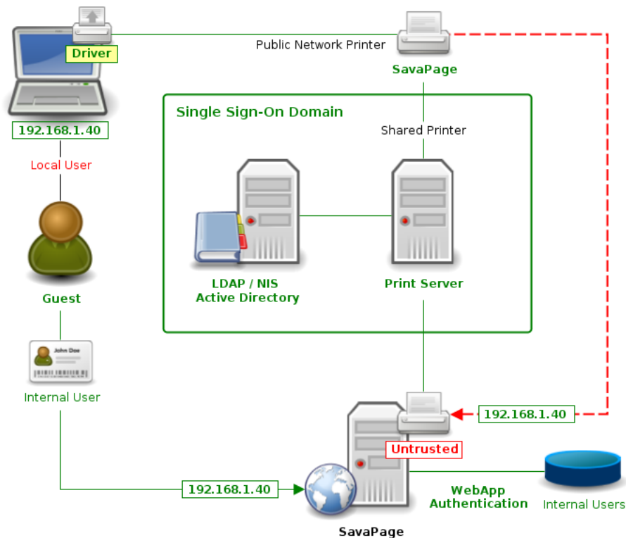
Figure 15.3. Authentication for Unauthenticated User
