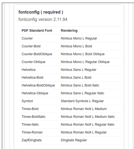
Figure 4.174. Admin Web App: About - PDF Standard Font Substitutes - 2/3
