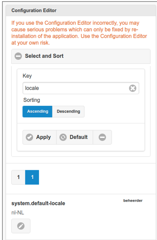
Figure 4.145. Admin Web App: Configuration Editor - List
