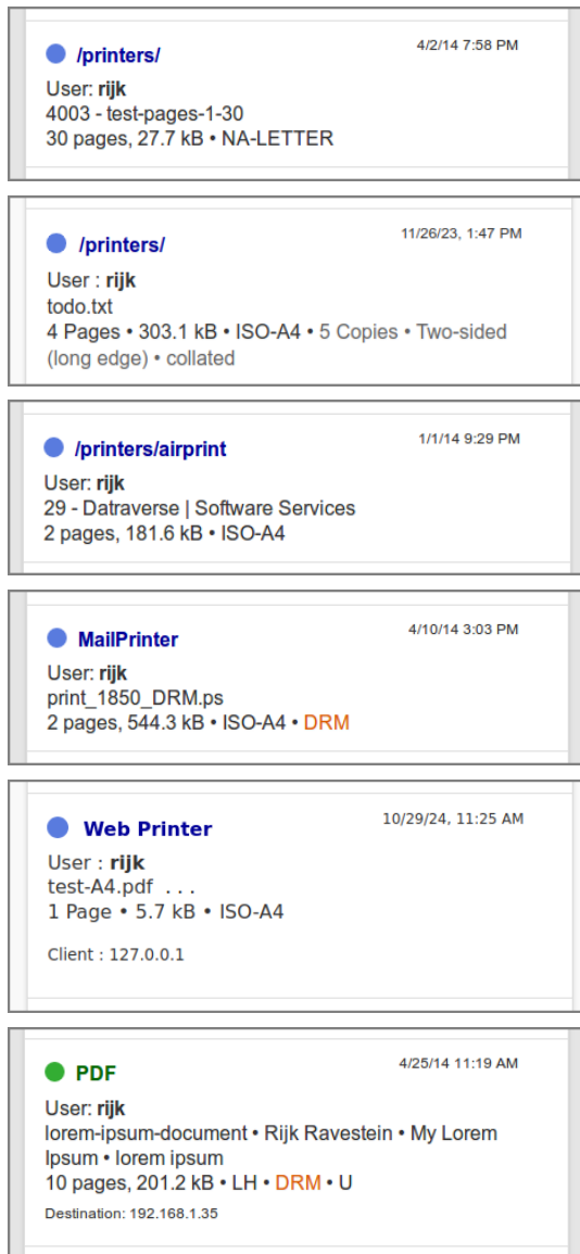
Figure 4.151. Admin Web App: Documents - Print-in - PDF out
