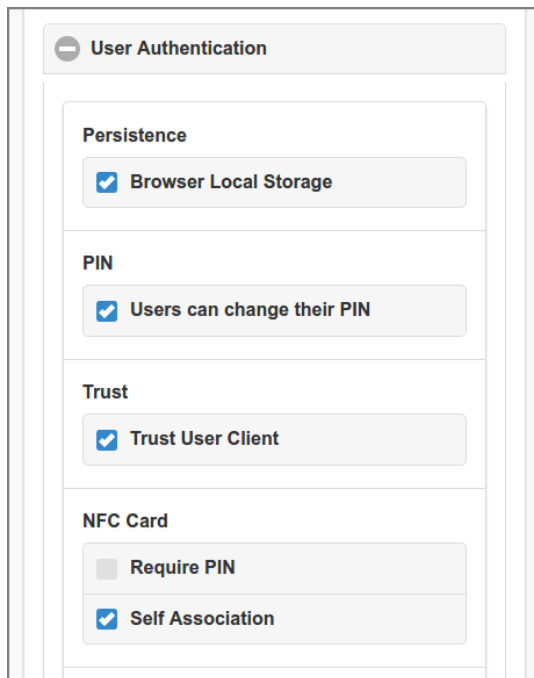
Figure 4.96. Admin Web App: Options - User Authentication
