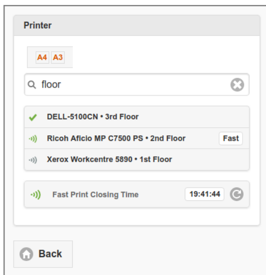
Figure 3.37. User Web App: Print - Select Printer
