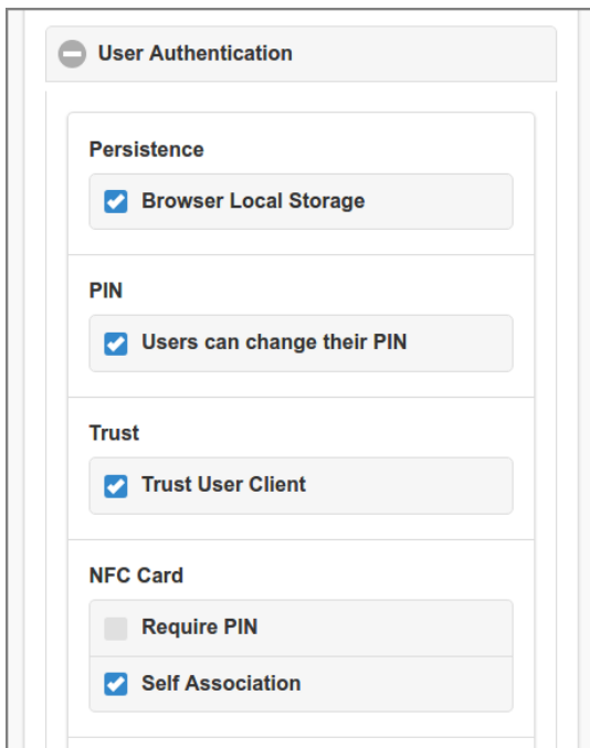
Figure 4.81. Admin Web App: Options - User Authentication
