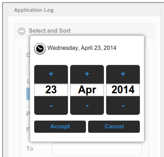
Figure 4.139. Admin Web App: Log - Select Date
