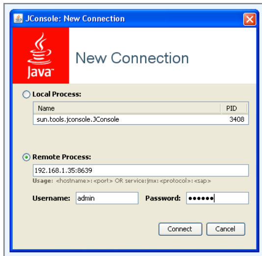
Figure 4.119. Connecting to Remote Process with JConsole
